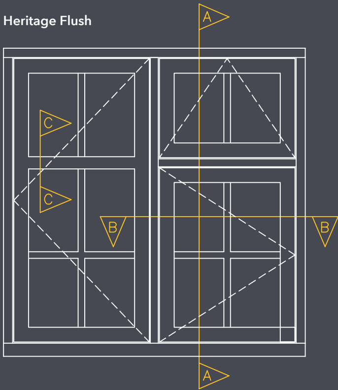
Horizontal Section B-B
