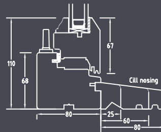
Vertical Section C-C
